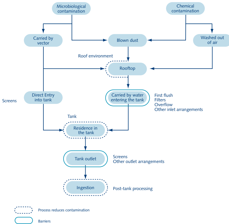
Figure 9.1. Contamination paths for roofwater harvesting
