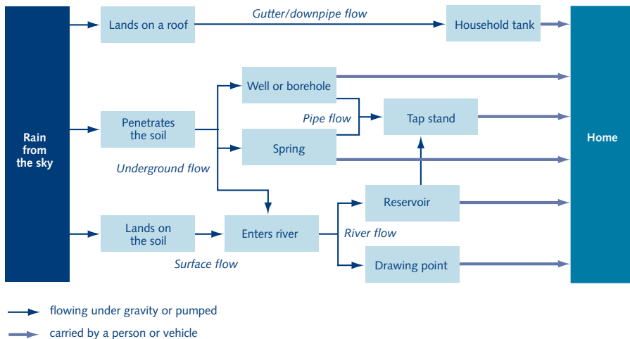
Figure 2.1. Common rural water supply techniques
