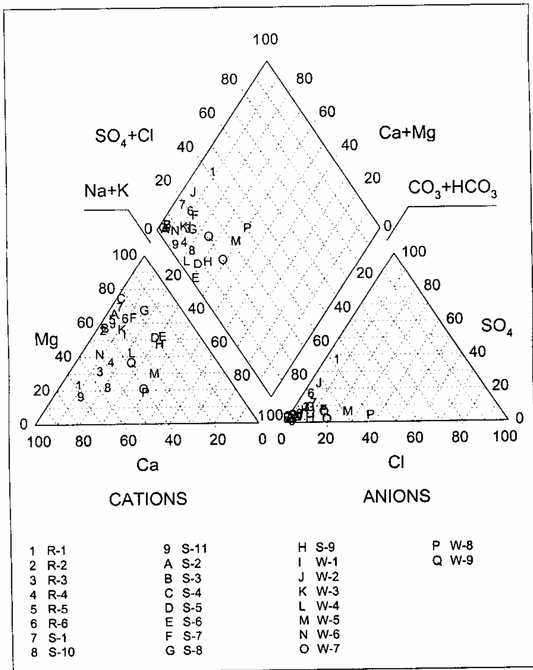
Fig 12 Piper Diagram (October, 1999).
