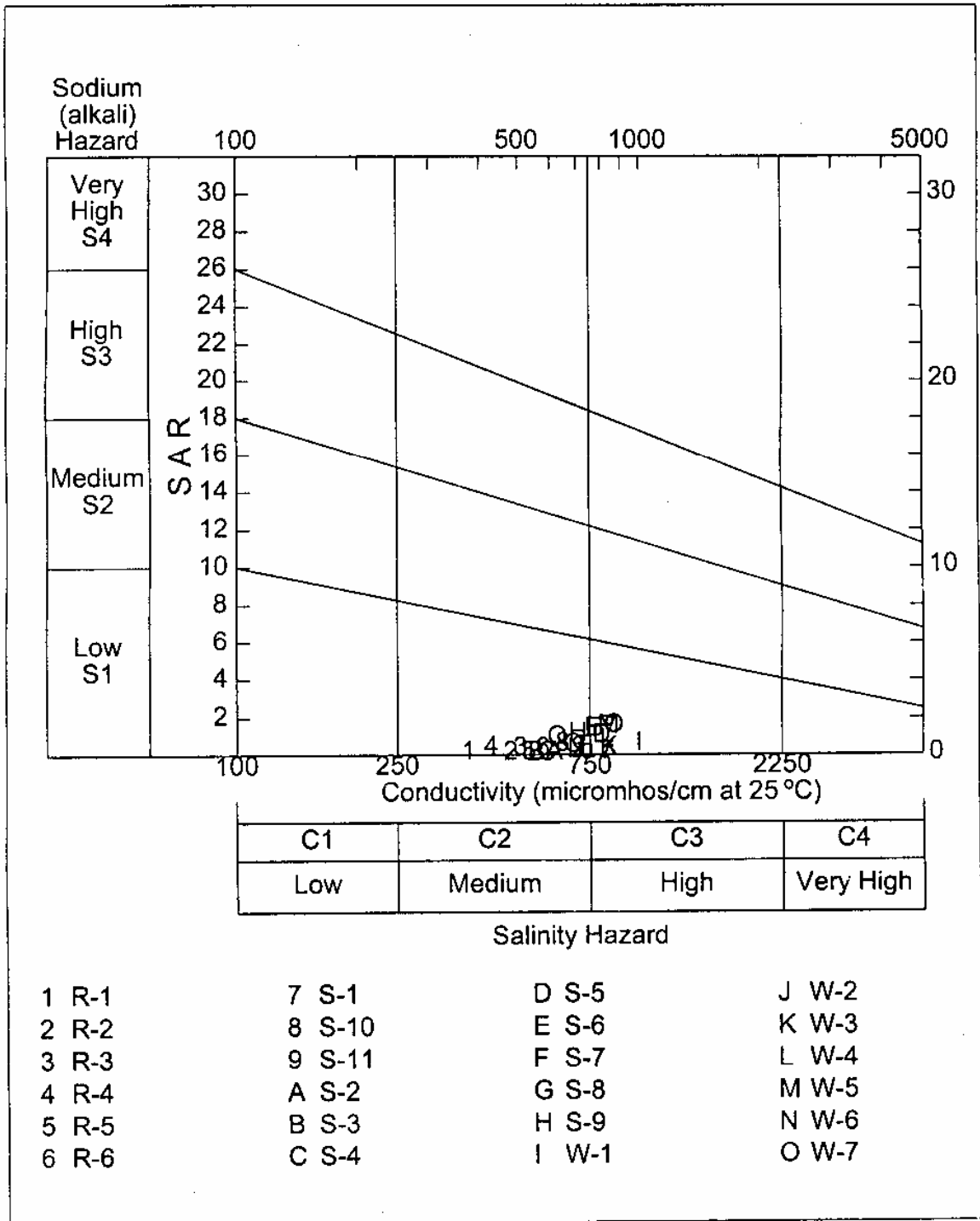
Fig 17. U.S. Salinity Diagram (October, 1999).
